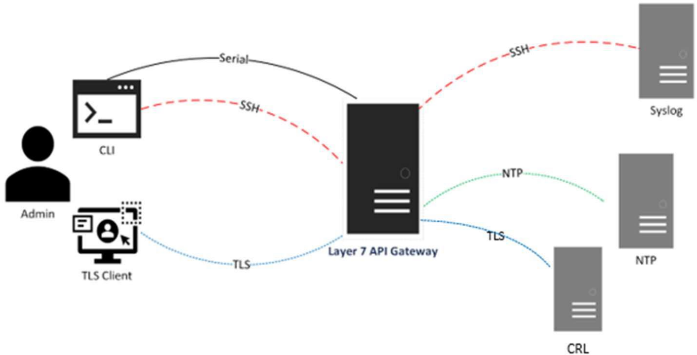
Figure 1: TOE Architecture
